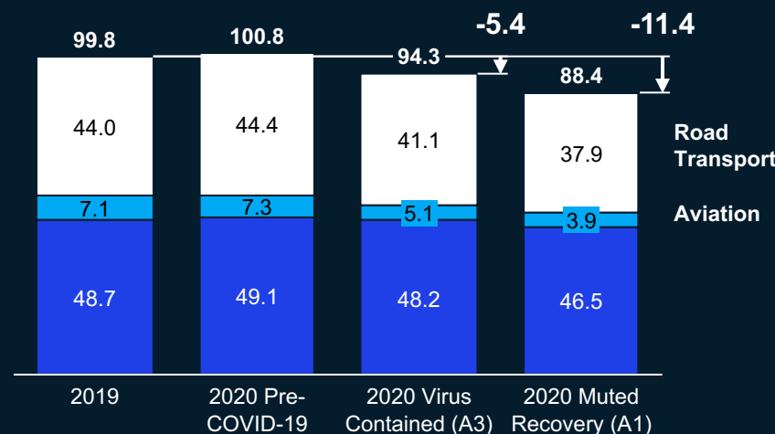
Oil demand, Mbd
